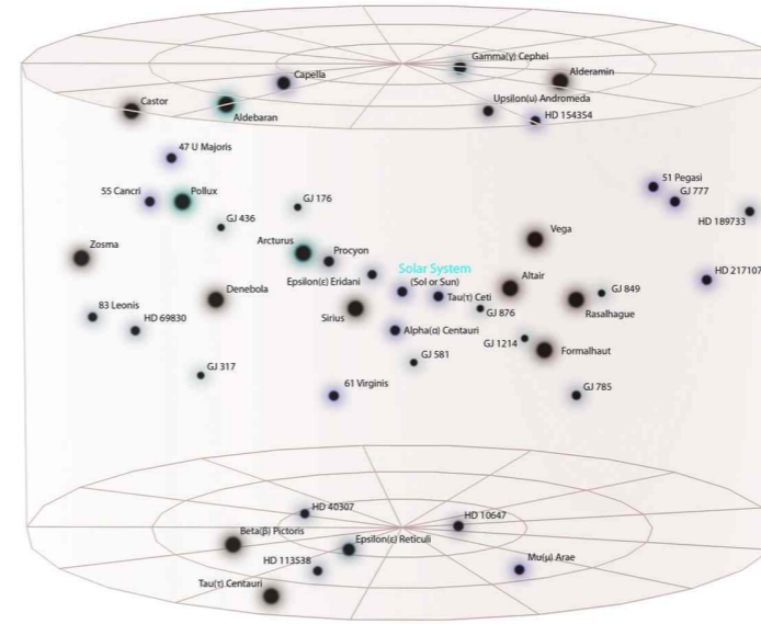
Solar Interstellar Neighborhood
