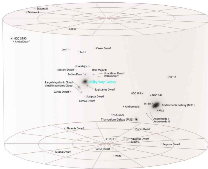
Local Galactic Group
