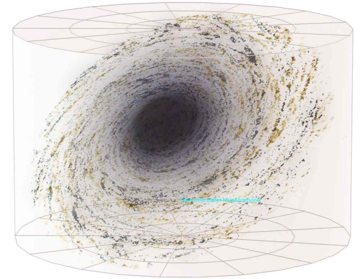
Milky Way Galaxy
