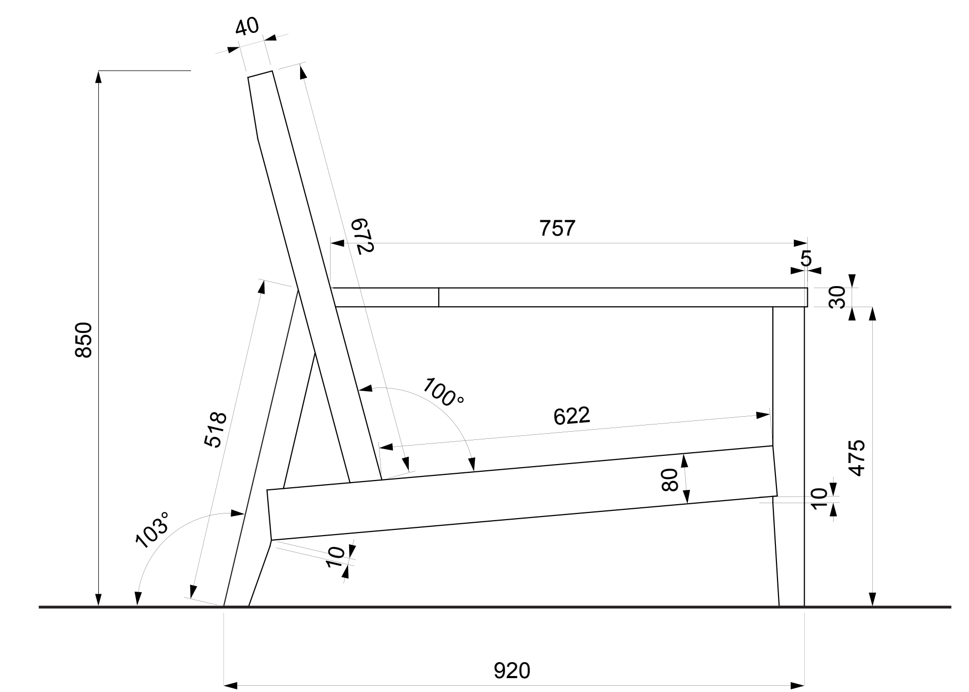
bokorys
