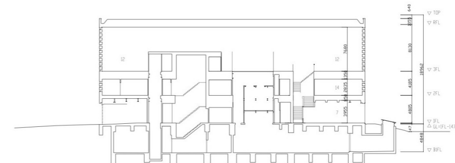
EAST-WEST SECTION (2) s:1/600
