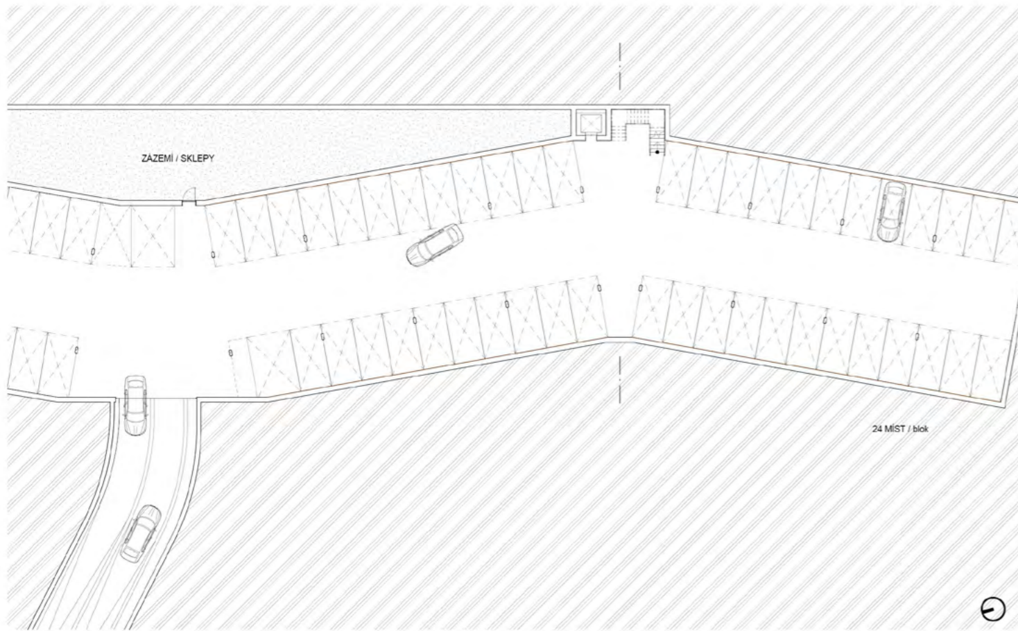
1PP M_1:200
