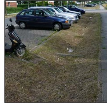
Photo 9. Kronsberg. Swale infiltration system with a sequential retention of water in small depressions.
